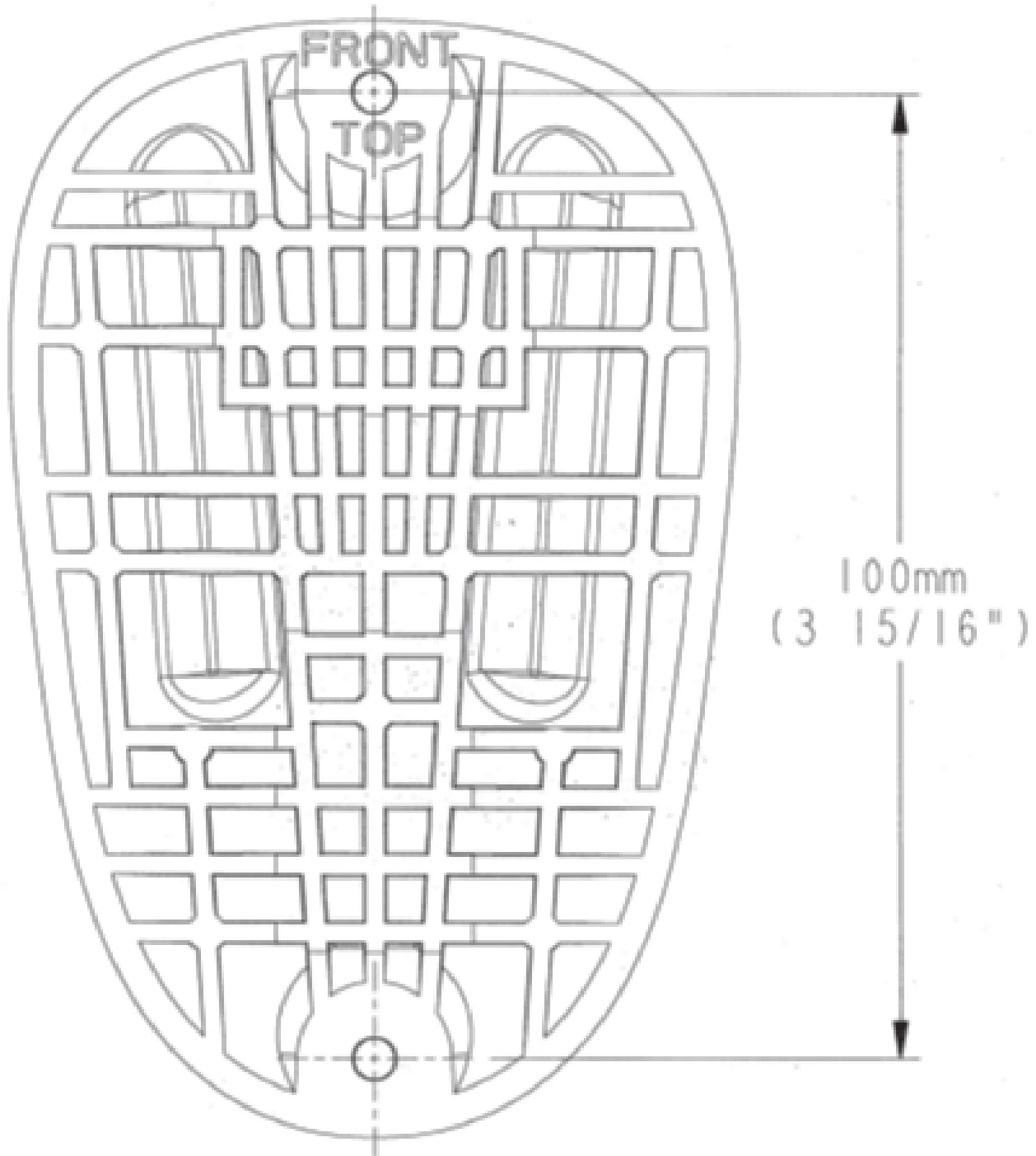
Figure 2. Drilling Template
