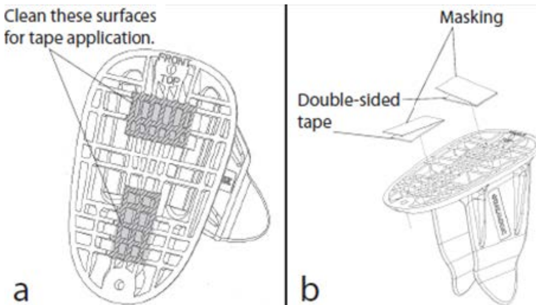
Figure 1. Applying the Double-Sided Tape
