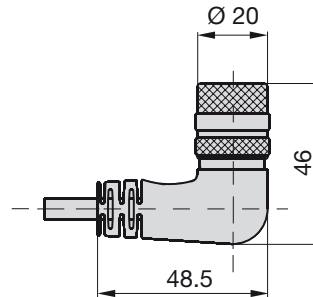
Fig. 8-13: Conector BKS-S233-PU-__
