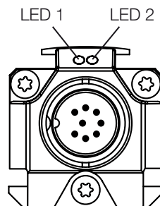
Fig. 3-2: Display LED BTL7
