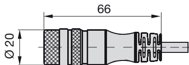
Fig. 8-12: Conector BKS-S232-PU-__
