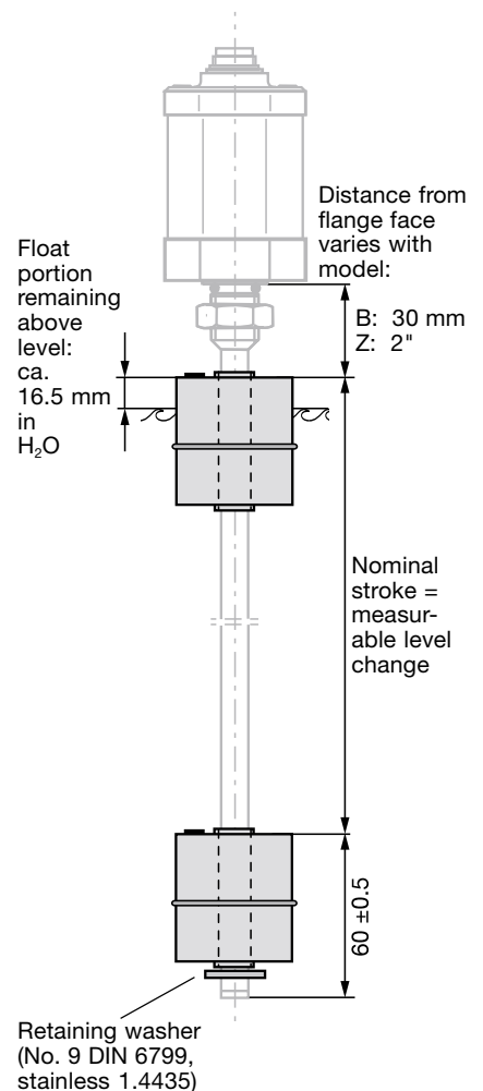
Fig. 3: Level detection with float BTL2-S-4414-4Z and transducer version BTL...B/Z...
