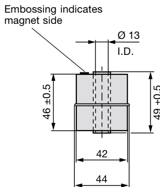
Fig. 1: Dimensions of float BTL2-S-4414-4Z
