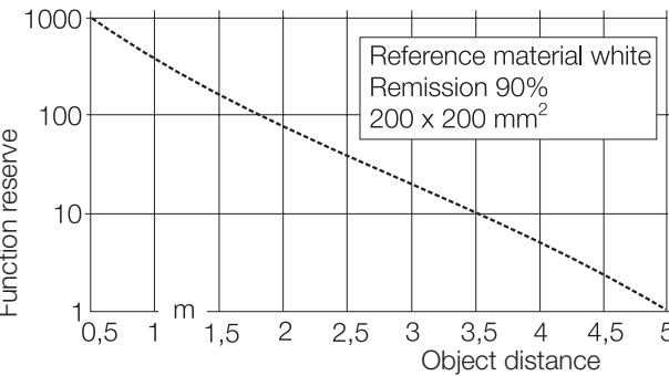
Fig. 3: Function reserve depending on distance to the object
