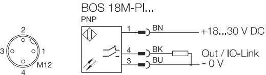
Fig. 2: Connection diagram, pinouts
