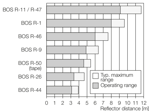
Fig. 9-1: Ranges
