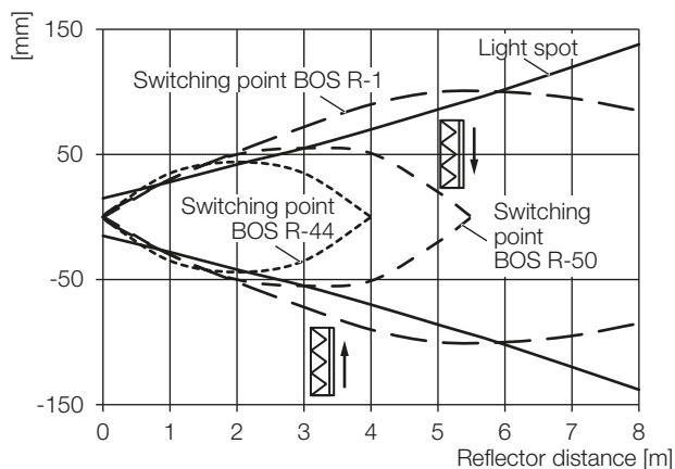
Fig. 9-3: Start-up curve
