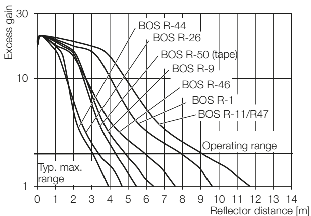
Fig. 9-2: Excess gain over distance
