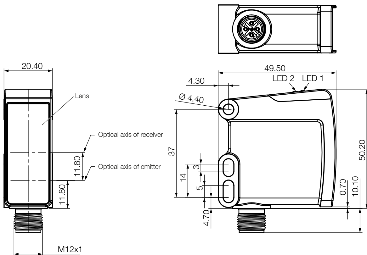
Fig. 4-1: Dimensions, design and function
