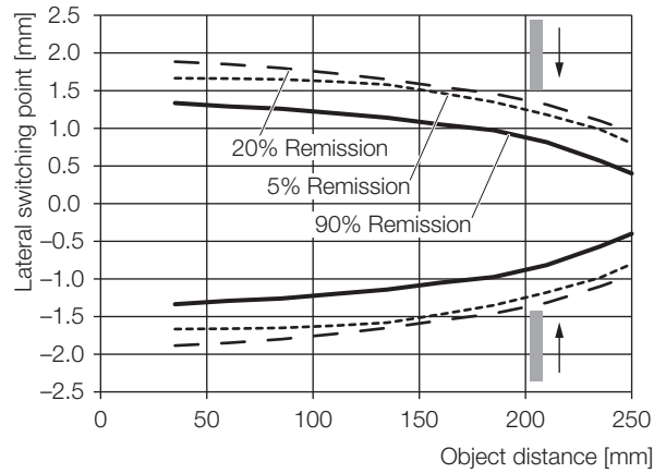
Fig. 9-4: Lateral switching point (...-LH10-...)
