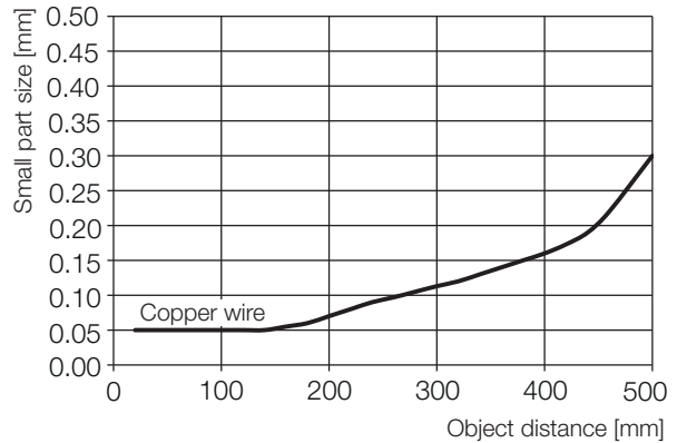
Fig. 9-11: Smallest recognizable part (...-LH11-...)
