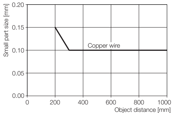
Fig. 9-12: Smallest recognizable part (...-LH12-...)
