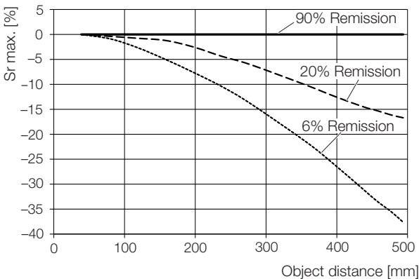
Fig. 9-2: Switching distance variation (...-LH11-...)
