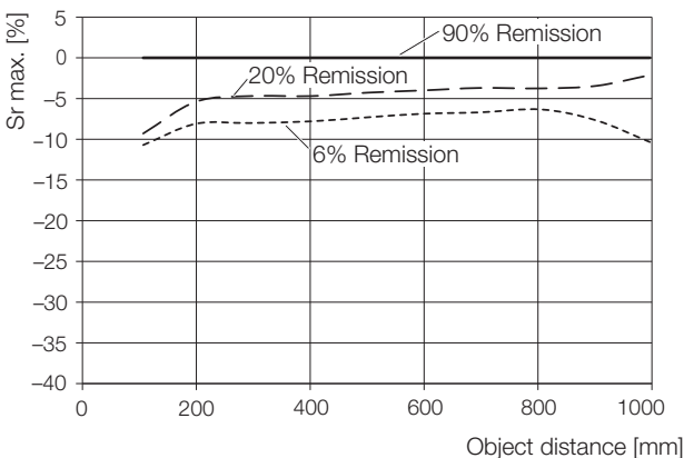
Fig. 9-3: Switching distance variation (...-LH12-...)
