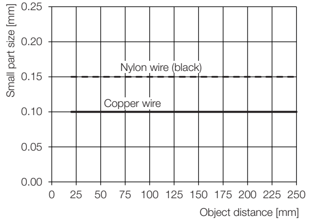
Fig. 9-10: Smallest recognizable part (...-LH10-...)
