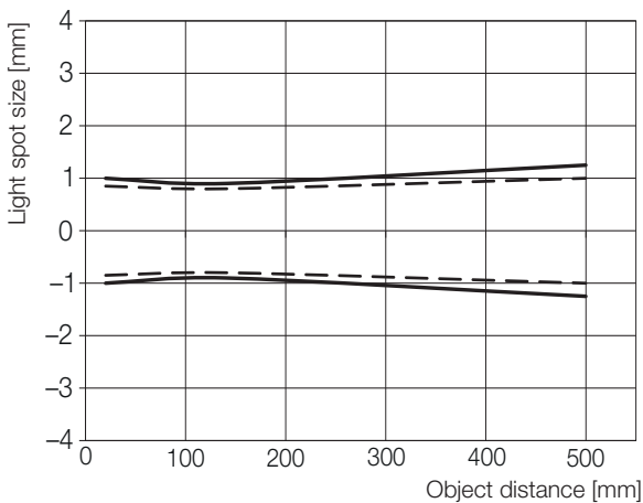
Fig. 9-8: Light spot size (...-LH11-...)
