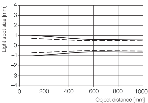
Fig. 9-9: Light spot size (...-LH12-...)
