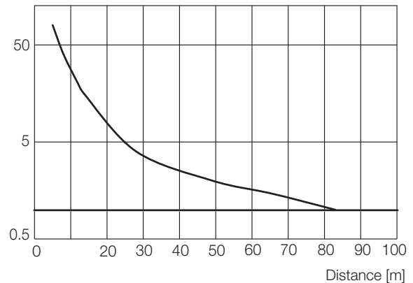
Fig. 9-17: Excess gain over distance (...-LS10/LE10-...)
