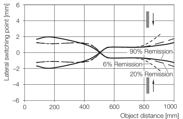
Fig. 9-6: Lateral switching point (...-LH12-...)
