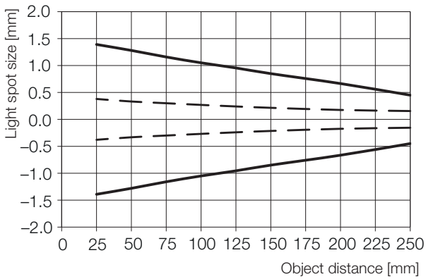
Fig. 9-7: Light spot size (...-LH10-...)
