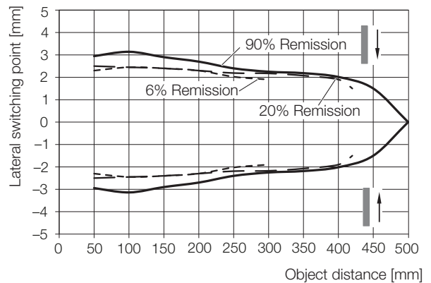
Fig. 9-5: Lateral switching point (...-LH11-...)
