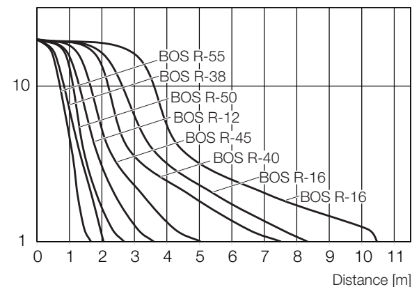
Fig. 9-15: Excess gain over distance (...-LK10-...)
