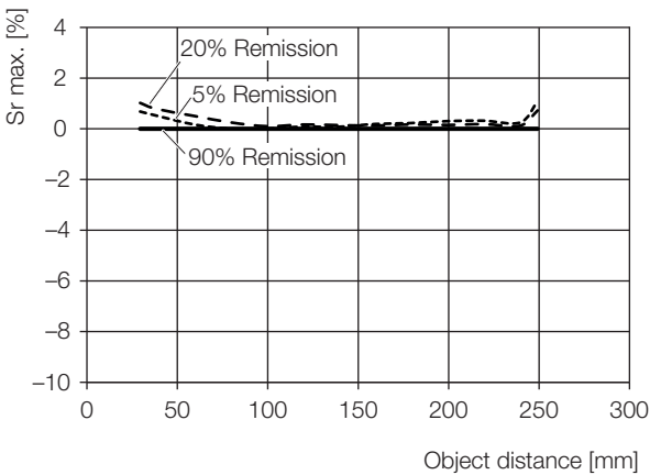
Fig. 9-1: Switching distance variation (...-LH10-...)
