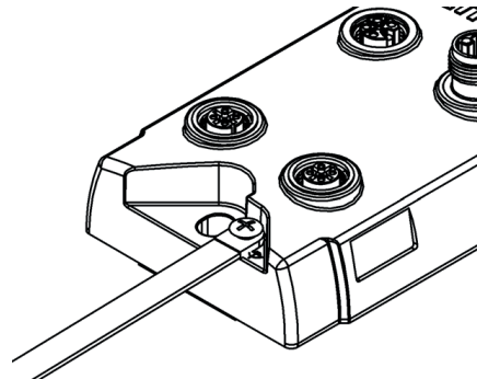
Fig. 5-4: Ground connection
