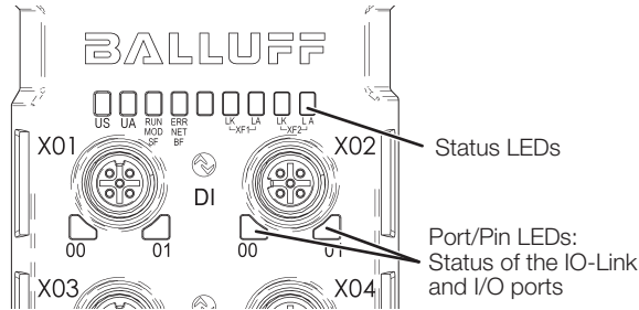
Fig. 4-3: Display elements
