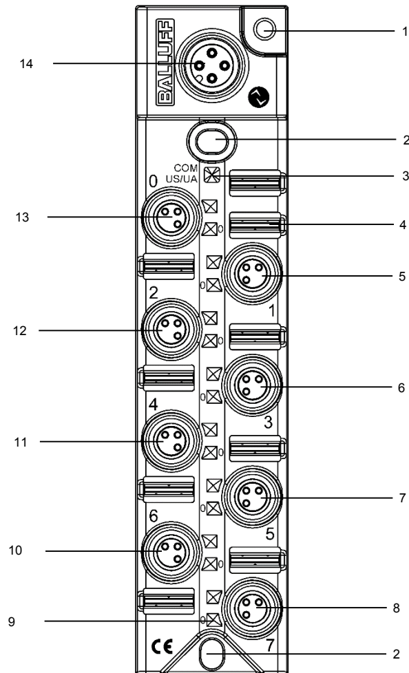
Figure 3-1: Connection overview BNI IOL-102-002-Z019
