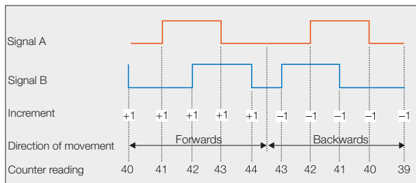
Fig. 2-23: BML output signals with period counter
