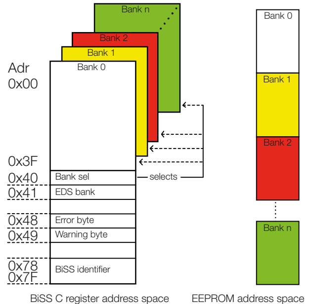
Fig. 2-9: BiSS C register address space
