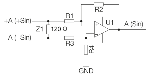
Fig. 2-14: Circuit example for follower circuit with analog output +A(+\sin) - (-A(-\sin))
