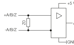
Fig. 2-24: Circuitry of subsequent electronics (RS422)
