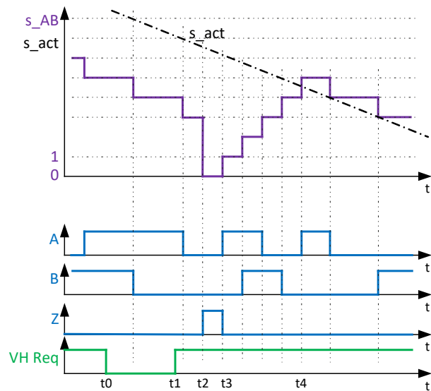
Fig. 2-11: Using input VH_{Req}
