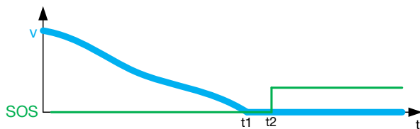
Fig. 2-18: Distance-time diagram for safe operating stop
