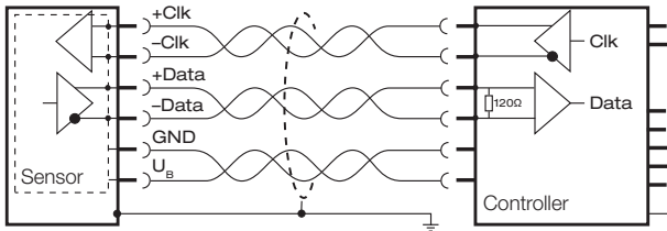
Fig. 2-5: Wiring example for a sensor with controller
