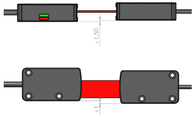
Fig. 3-2: Maximum permissible offset
