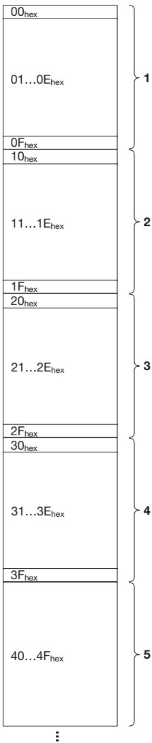
Figure 13: Example for a total buffer size of 80 bytes (4 × 16 bytes: heads H1 to H4, 16 bytes: IO-Link)
