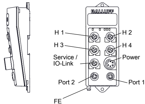
Figure 4: Electrical Connections
