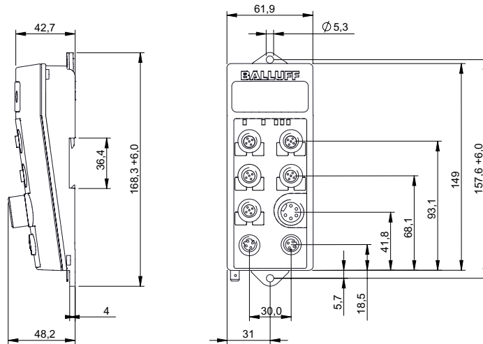
Figure 5: Dimensions in mm
