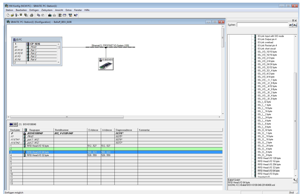
Figure 10: Configuring read/write heads
