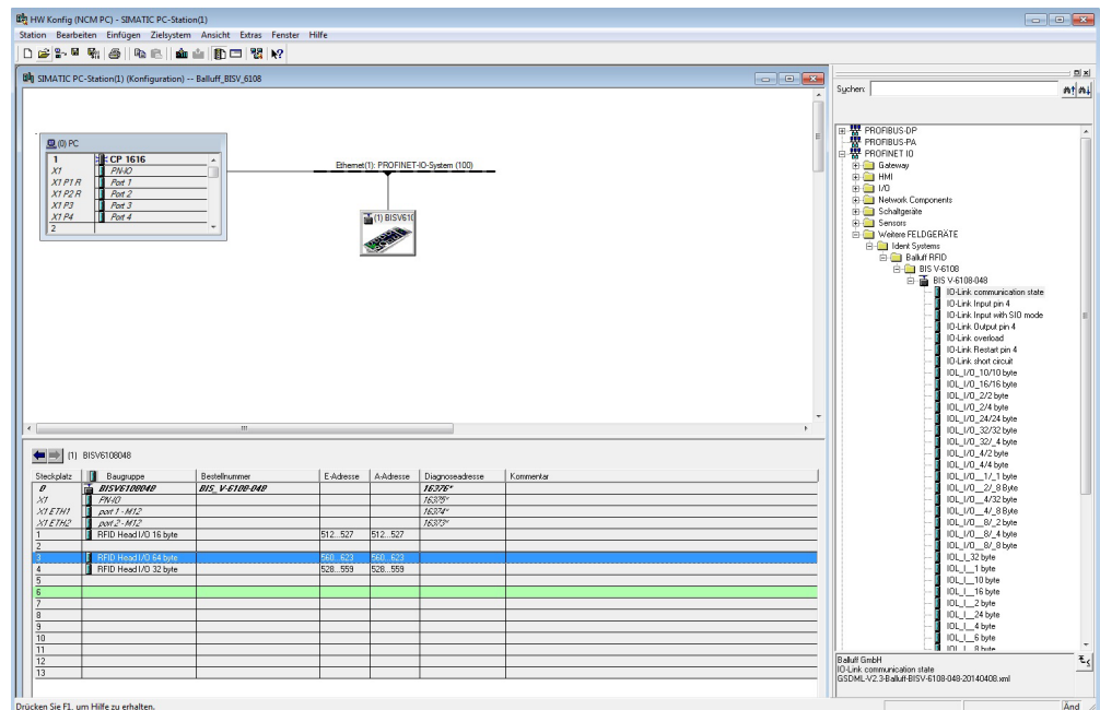
Figure 12: Plugging in the IO-Link module
