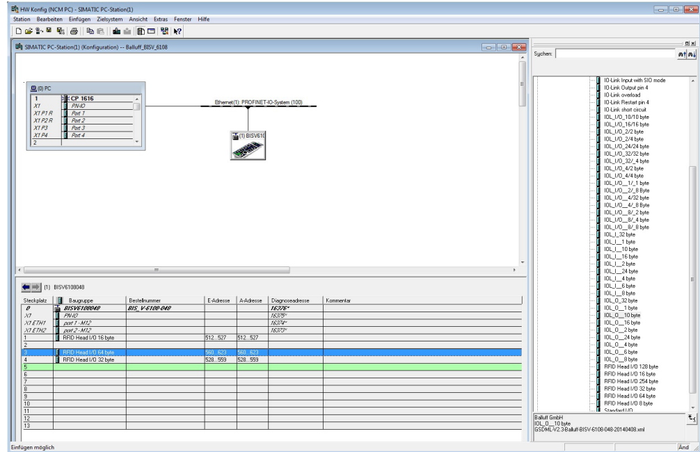
Figure 11: Selecting the IO-Link module
