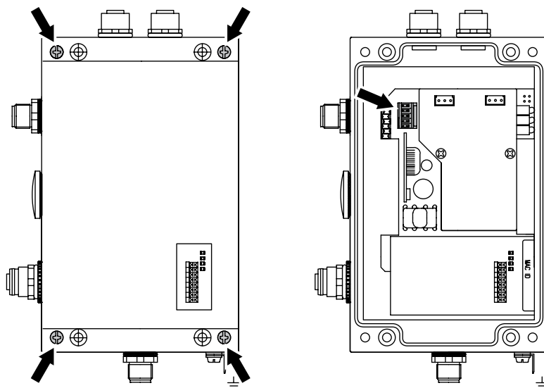
Fig. 6: Changing the EEPROM
