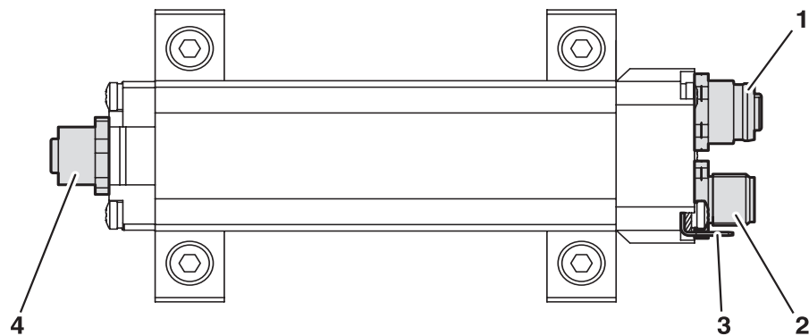
Fig. 2: Electrical connection
