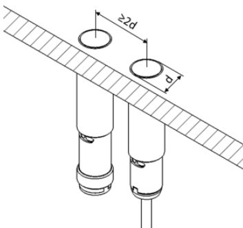
Fig. 4-2: Installing flush-mount sensors
