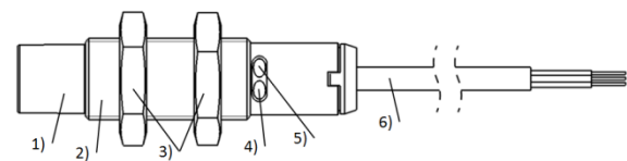
Fig. 3-2: Cable version construction, 1) Sensing surface, 2) Mounting thread M12x1, 3) Fastening nuts, 4) Sensor state indicator (green LED), 5) Switching state indicator (yellow LED), 6) Connection cable
