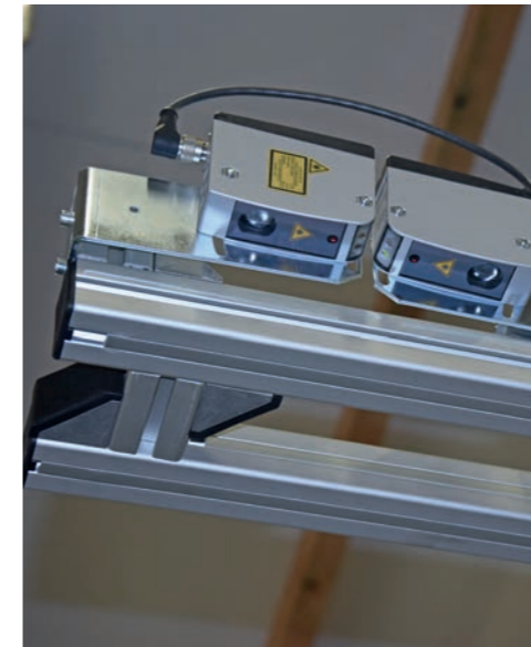
COBOT GUIDANCE WITH PHOTOELECTRIC DISTANCE SENSORS
