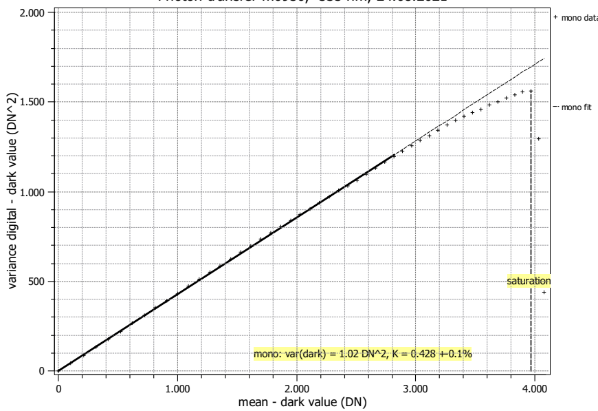
Photon transfer m0950, 535 nm, 24.08.2021
